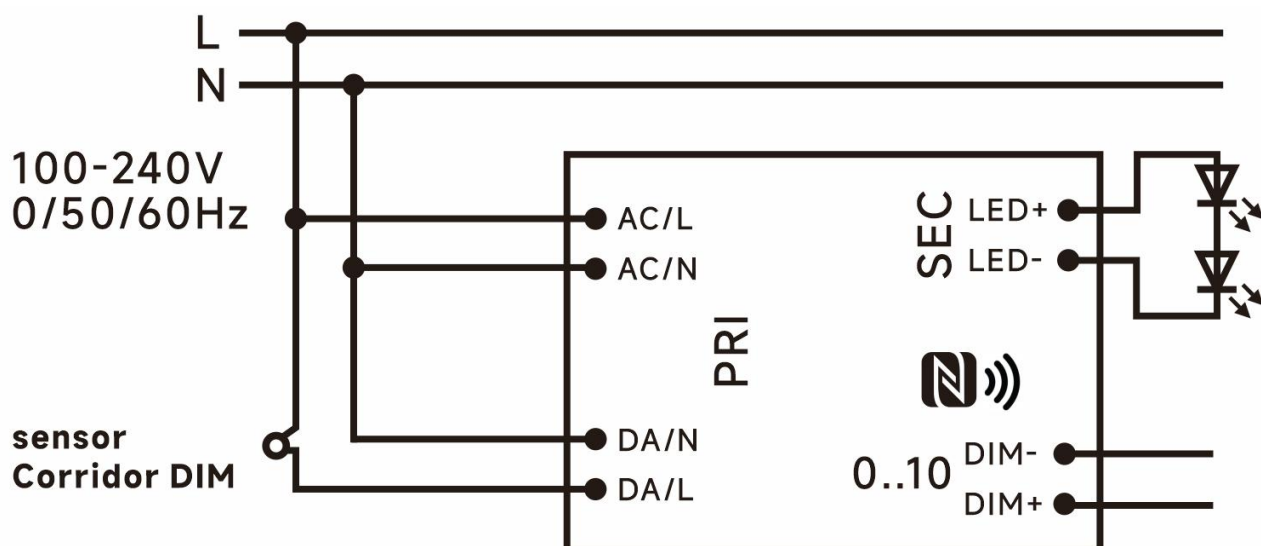
Corridor DIM dimming application
