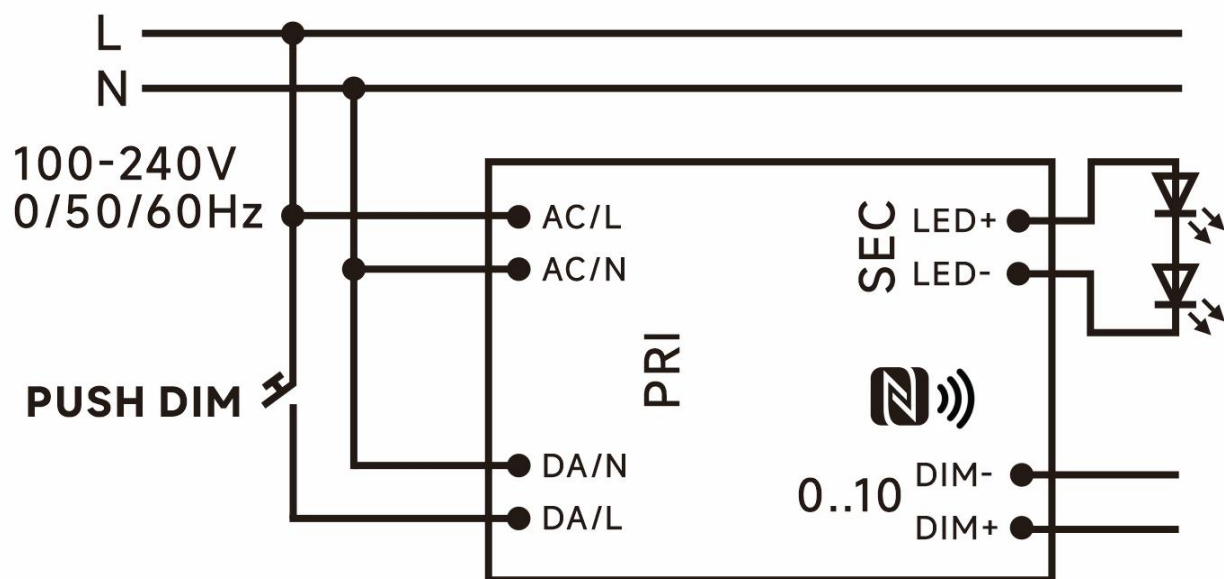
PushDIM dimming application
